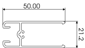
ROUGE SASH HEAD & SILL W34207
