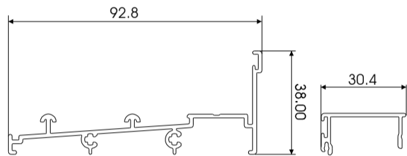
ROUGE SILL RAIL TRIPLE TRACK W34635
