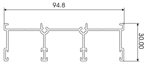
ROUGE HEAD RAIL TRIPLE TRACK W34633
