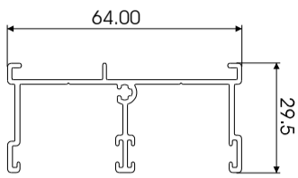
ROUGE FRAME HEAD W34206
