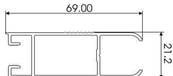
ROUGE STILE LOCK W56834
