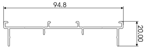
ROUGE JAMB RAIL TRIPLE TRACK W34634
